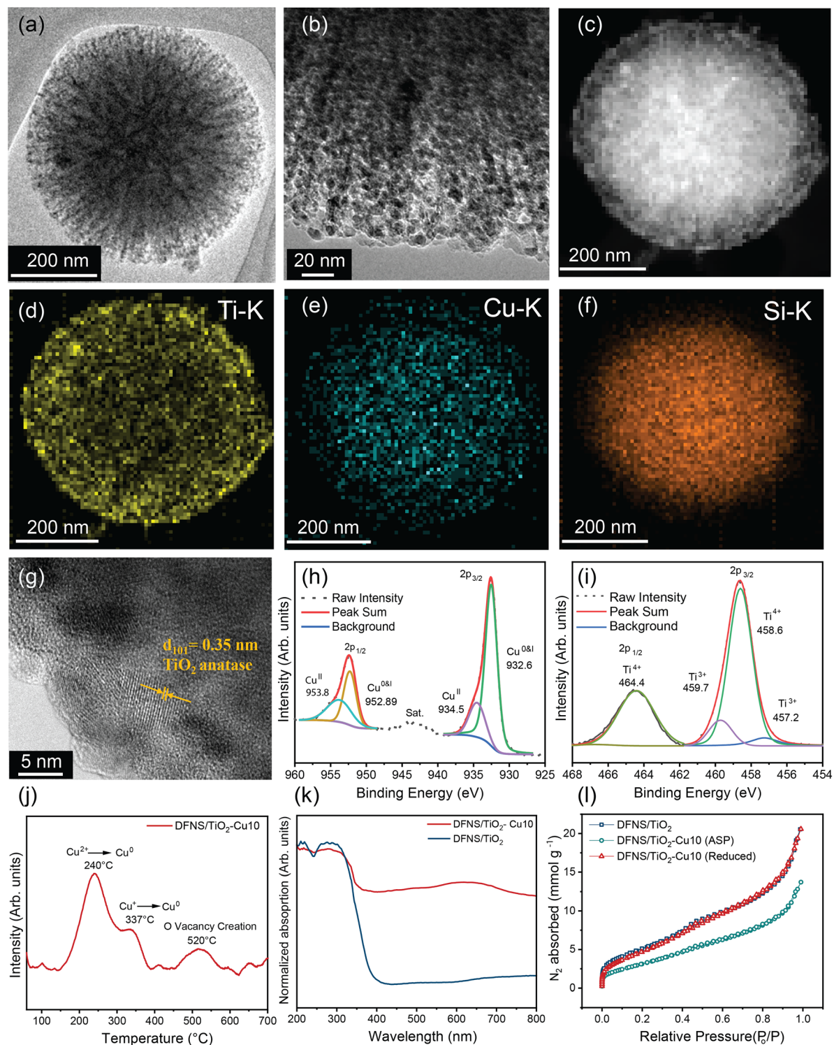
Fig. 2 DFNS/TiO 2 -Cu10 catalyst characterisation, (a) and (b) HRTEM images; (c) HAADF-STEM images; (d)–(f) STEM-EDS elemental mapping; (g) HRTEM image showing anatase phase of TiO 2 ; XPS spectra for (h) Cu 2p and (i) Ti 2p; (j) TPR profile of DFNS/TiO 2 -Cu10 as prepared (ASP) catalyst; (k) UV-Vis DRS (diffuse reflectance spectra) for DFNS/TiO 2 and DFNS/TiO 2 -Cu10 (reduced) catalyst; (l) N 2 sorption isotherms for DFNS/TiO 2 , DFNS/TiO 2 -Cu10 (ASP) and reduced catalyst.
