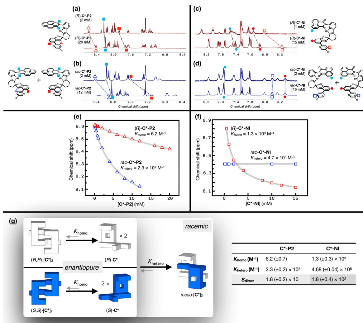
Fig. 3 1 H NMR (400 MHz, T = 298 \text{ K} ) spectra of (a) ( R )- C * -P2 , (b) rac - C * -P2 , (c) ( R )- C * -NI , and (d) rac - C * -NI obtained at two different concentrations are shown for qualitative comparison. For a full analysis of the concentration-dependence, changes in the chemical shifts of the pyridyl proton resonances (annotated by blank triangles or squares in the chemical structures) are plotted as a function of the concentration of (e) ( R )- C * -P2 and rac - C * -P2 , or (f) ( R )- C * -NI and rac - C * -NI in CDCl 3 at T = 298 \text{ K} . The overlaid gray lines in (e) and (f) are theoretical fits from non-linear least-squares regression, taking into account both homochiral dimerization ( K_{\text{homo}} ) and heterochiral dimerization ( K_{\text{hetero}} ), as described in (g). The solution equilibrium, schematically shown in (g), is dictated by the dimerization constants K_{\text{homo}} and K_{\text{hetero}} in the table on the right, which were obtained by numerical global fitting. The selectivity coefficient S_{\text{dimer}} is defined as K_{\text{hetero}}/(2K_{\text{homo}}) .
