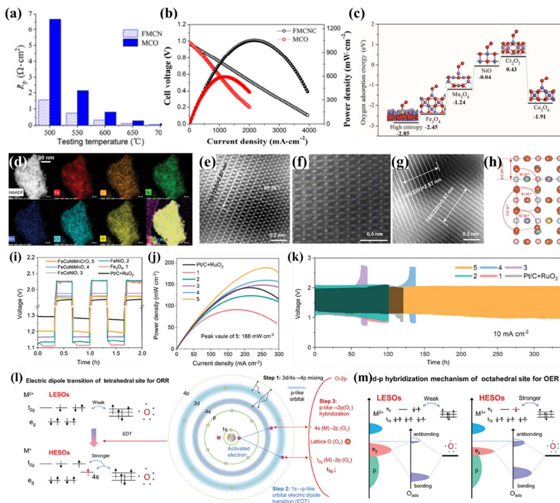
Fig. 9 HESSs for the ORR. (a) The polarization resistance ( R_p ) values of the cell using \text{Fe}_{0.6}\text{Mn}_{0.6}\text{Co}_{0.6}\text{Ni}_{0.6}\text{Cr}_{0.6}\text{O}_4 (FMCNC) and \text{Mn}_{1.6}\text{Cu}_{1.4}\text{O}_4 (MCO) cathodes tested at different temperatures, (b) the fuel cell performance, and (c) \text{O}_2 adsorption energy on the surface of HES, \text{Fe}_3\text{O}_4 , \text{Mn}_3\text{O}_4 , \text{Co}_3\text{O}_4 , \text{NiO} , and \text{Cr}_2\text{O}_3 . 49 (d) STEM image and EDS mapping, (e–g) HAADF-STEM images and (h) the corresponding simulated model of HESS ( \text{FeCoNiMnCrO} ), (i) charge-discharge curves of ZABs at initial three cycles at 10\ \text{mA}\ \text{cm}^{-2} using different spinels and commercial catalysts (Pt/C and \text{RuO}_2 ) electrodes, (j) powder density, (k) long-term cycling curves at 10\ \text{mA}\ \text{cm}^{-2} , (l) high-entropy induced robust electric dipole transition in tetrahedral sites for the ORR, and (m) high-entropy induced strong d–p hybridization of octahedral sites for the OER. Reproduced with permission. 137 Copyright 2024, John Wiley and Sons.
