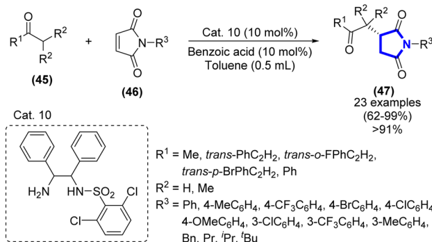
Scheme 13 Synthesis of pyrrolidines catalyzed by Cat. 10 .
