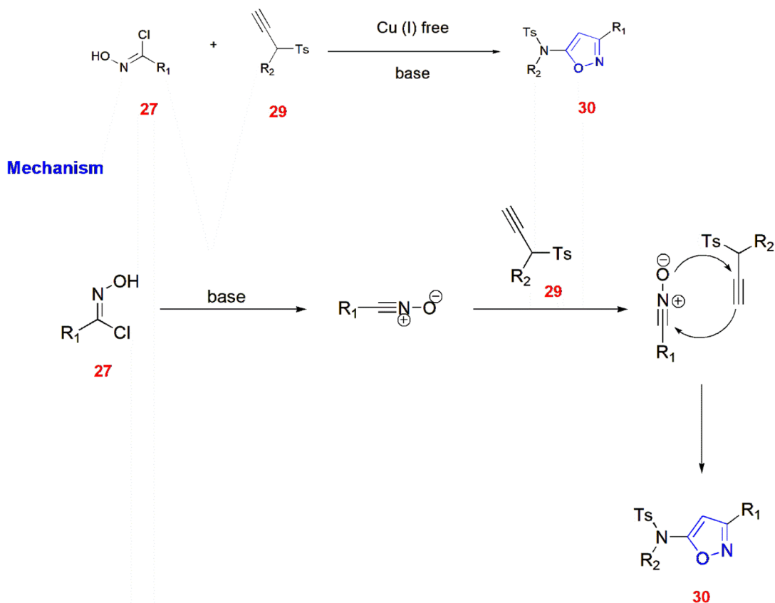
Scheme 9 Synthesis of isoxazoles 30 from nitrile oxides and nymides 29.
