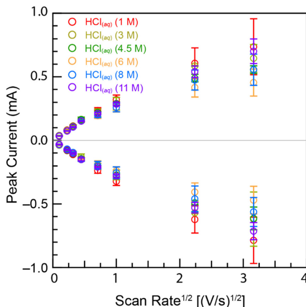
Fig. 6 Peak current ( i p ) from cyclic voltammetric measurements made on plutonium (16.7 mM) in HCl (aq) (1–11 M) solutions plotted as a function of scan rate (0.01–10 V s -1 ). Error bars are the standard deviation from three replicates.
