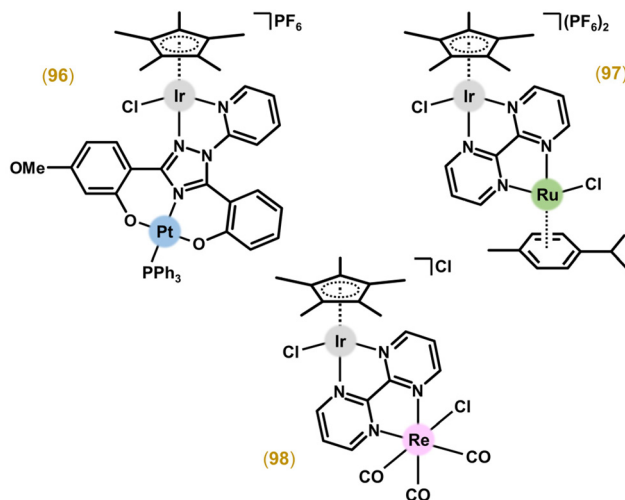
Fig. 24 Structural formulas of heterometallic complexes 96–98.
