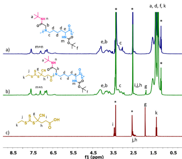
Fig. 1 1 H-NMR spectrum of (a) Boc-P \epsilon LL, (b) Boc-P \epsilon LL-TTC, and (c) pure CEPA in DMSO-d 6 confirming the success in the synthesis of Boc-P \epsilon LL-TTC using the Ugi multicomponent reaction, * indicates the residual solvent.
