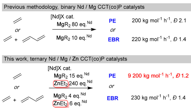
Scheme 1 Implementation of the CCTP of ethylene and CCTcoP of ethylene and butadiene mediated by binary or ternary Nd-based catalysts. [Nd] corresponds to the metal center and its ligands (Me 2 Si(C 13 H 8 ) 2 ), [Nd]X = \{[(\text{Me}_2\text{Si}(\text{C}_{13}\text{H}_8)_2)\text{Nd}(\mu\text{-BH}_4)[(\mu\text{-BH}_4)\text{Li}(\text{THF})]]_2\} .
