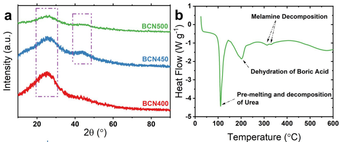
Fig. 2 XRD patterns of B_xC_yN_z formed at 400, 450, and 500 °C along with the XRD pattern of BCN (a), and the calorimetric (DSC) curve recorded during the formation of B_xC_yN_z from its precursors (b).
