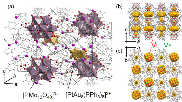
Fig. 1 (a) Crystal structure of PtAu8-PMo12 . 27 Void analysis of PtAu8-PMo12 in the (b) ac -plane and (c) ab -plane. Void space (in yellow) is depicted with a probe radius of 1.2 Å using the CSD Mercury software. 29
