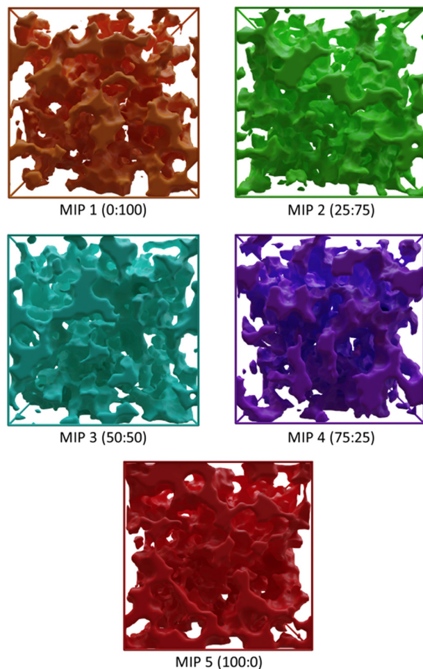
Fig. 7 Visualization of the computed free volume within the MIP structures (solvent removed) for each solvent composition: 0:100, 25:75, 50:50, 75:25, and 100:0 DMSO:ACN. These images (from the MeshSA analysis) show regions of accessible void space (coloured surfaces) within the polymer matrix.
