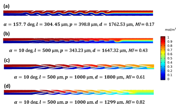
Fig. 8 Progression of mixing performance in the micromixer with parallelogram barriers through the BO process for Re = 5, showing concentration profiles in the micromixer across four iterations. (a) Initial parameter set, (b) and (c) intermediate iterations, and (d) final iteration with the optimal parameter set.
