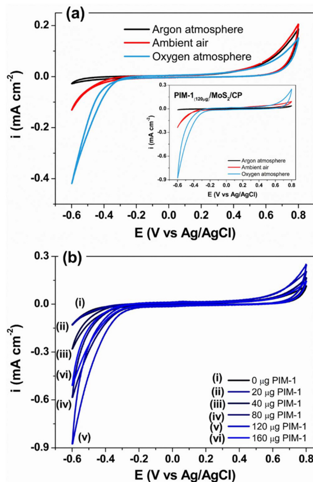
Fig. 5 (a) Cyclic voltammograms (scan rate 50 mV s -1 ) for MoS 2 /CP and PIM-1 (120 μg) /MoS 2 (inset) in 0.1 mol L -1 phosphate buffer pH 7 for different gas environments. (b) Cyclic voltammograms (scan rate 50 mV s -1 ) in ambient air for MoS 2 /CP with different amounts of PIM-1 nanoparticles deposits (20–160 μg).
