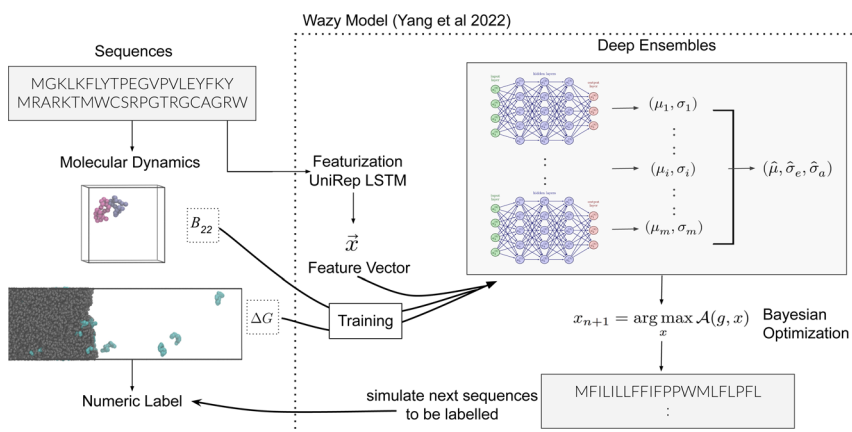
Fig. 1 Schematic overview of the active learning framework for predicting peptides using Bayesian Optimisation (BO) and Molecular Dynamics (MD) simulations: (A) MD simulations of protein chains to compute second virial coefficient ( B_{22} ) and partition free energy ( \Delta G ) for model training. This initial sample is fed to the wazy BO package, 25 which utilises UniRep LSTM, 24,26 to parse the protein sequence into a feature vector \vec{x} . Deep ensemble training on feature vectors and computed properties to establish sequence–property relationships. To choose which sequences the model would benefit the most from, an acquisition function \mathcal{A} is used to rank and suggest the next set of sequences. The suggested sequences are simulated again, generating new data for subsequent training cycles. This iterative process helps the model learn the sequence–property relationship with fewer examples and simultaneously explore sequence space regions that contain proteins with the most extreme values of the property we studied.
