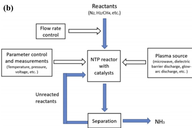
Fig. 14 (a) Summative scheme of the main reactions between molecules and atoms. Figure has been reproduced from ref. 133 with permission from Wiley © 2019 Wiley-VCH Verlag GmbH & Co. KGaA, Weinheim. (b) A flow diagram of the non-thermal plasma \text{NH}_3 synthesis process. 129 Figure has been reproduced from ref. 129 with permission from Elsevier © 2018 Elsevier.
