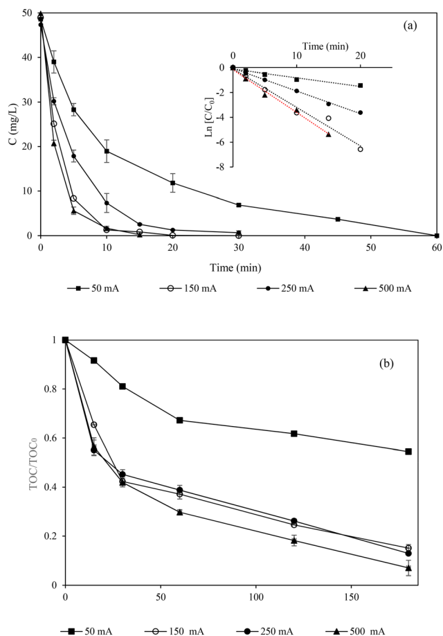
Fig. 2 Effect of the applied current intensity on miconazole degradation (a) and mineralization (b) during electro-Fenton treatment [ \text{Na}_2\text{SO}_4 ] = 50 mM, \text{Fe}^{2+} = 0.2 mM and pH = 3.0.
