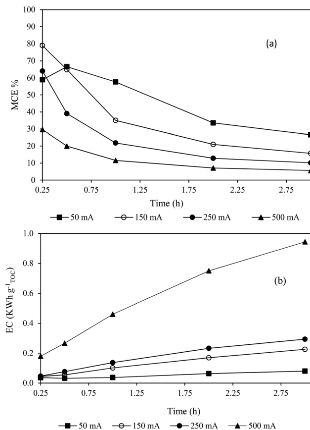
Fig. 3 Mineralization current efficiency (% MCE) (a) and energy consumption ( \text{EC}_{\text{TOC}} ) (b) as a function of electrolysis time of 50 \text{mg L}^{-1} of miconazole corresponding to 25.95 \text{mg L}^{-1} initial TOC by electro-Fenton under operating conditions of [ \text{Na}_2\text{SO}_4 ] = 50 mM, \text{Fe}^{2+} = 0.2 mM and pH = 3.0.
