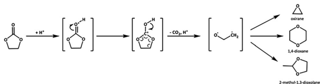
Fig. 5 Proposed reaction scheme for \text{H}^+ -catalyzed decomposition of EC. The reaction branches out after the formation of \text{CO}_2 and \text{HO}-\text{CH}_2-\text{CH}_2\cdot moieties from the ring opening process, to form a series of ether-based molecules and polymers. The scheme shows molecules detected in our experiments only.
