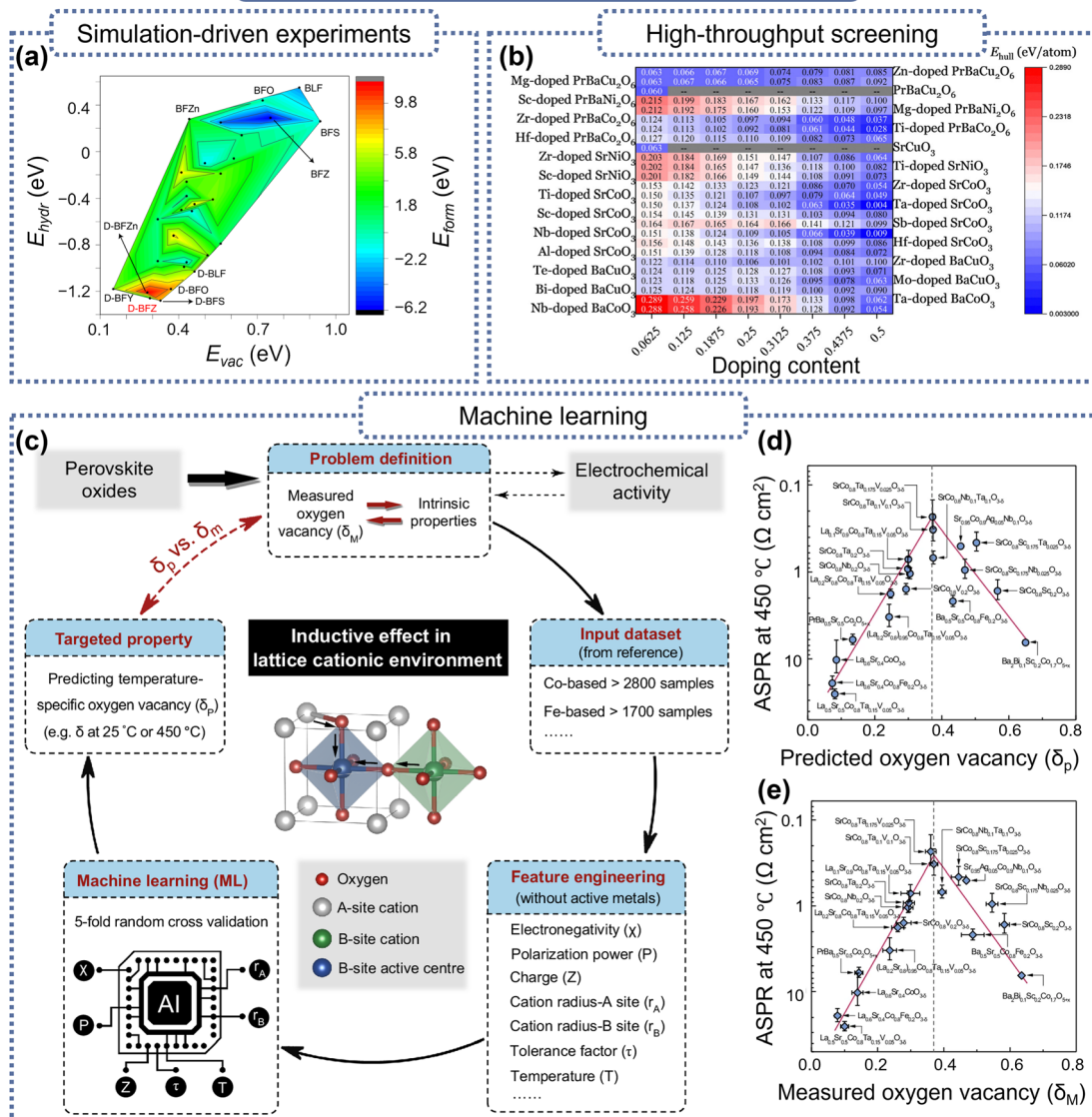
Fig. 13 (a) Plot of computed E_{\text{form}} against E_{\text{vac}} and E_{\text{hydr}} for BFO and its derivative materials (dots). Reproduced with permission. 34 Copyright 2022, Springer Nature. (b) Promising perovskite candidates with exceptional thermodynamic stability. Reproduced with permission. 237 Copyright 2024, Royal Society of Chemistry. (c) Workflow of oxygen vacancies prediction, and (d) and (e) the measured and predicted ASR. Reproduced with permission. 81 Copyright 2024, Springer Nature.
