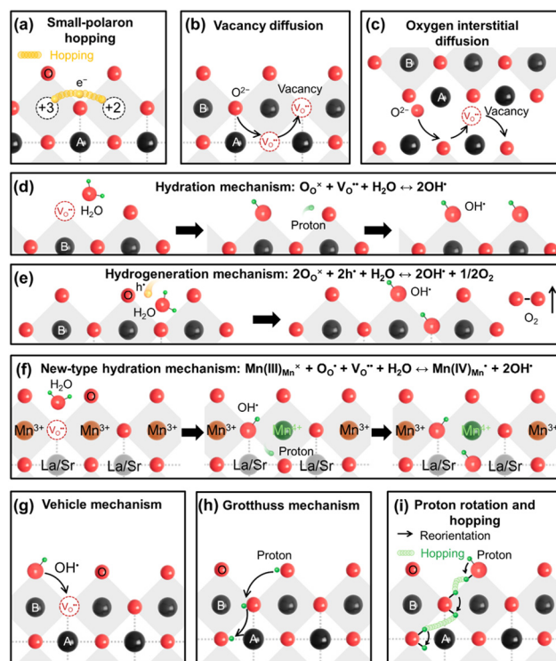
Fig. 4 Charge conduction mechanism (red spheres: \text{O}^{2-} ; yellow spheres: \text{e}^- ; green spheres: \text{H}^+ ). (a) \text{e}^- conduction mechanism: small-polaron hopping mechanism. \text{O}^{2-} conduction mechanisms: (b) vacancy diffusion mechanism and (c) oxygen interstitial diffusion mechanism. \text{H}^+ uptake mechanism: (d) hydration mechanism, (e) hydrogeneration mechanism, and (f) new-type hydration mechanism; \text{H}^+ transfer mechanism: (g) vehicle mechanism, (h) Grotthuss mechanism, and (i) \text{H}^+ reorientation and hopping for Grotthuss mechanism.
