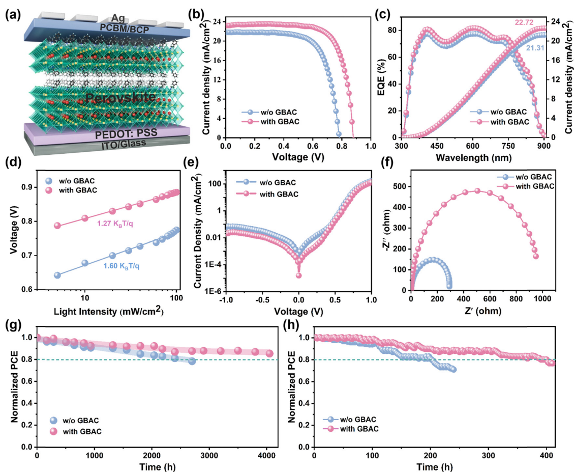
Fig. 5 (a) Schematic illustration of the device structure for tin PSCs. (b) J-V curves of the champion tin PSCs without and with GBAC. (c) EQE spectra of the corresponding tin PSCs. (d) Open-circuit voltage depends on the light intensity. (e) Dark current and (f) EIS results of tin PSCs without and with GBAC. (g) Long-term shelf stability and (h) operational stability of tin PSCs without and with GBAC (in a \text{N}_2 environment).
