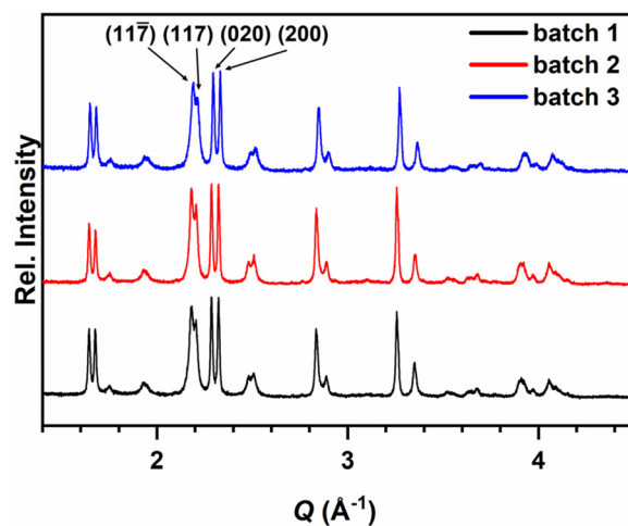
Fig. 3 XRD patterns of \text{La}_4\text{Ni}_3\text{O}_{8.4}\text{F}_{3.5} from different batches. The indices are given for the (117)/(11-7) and (200)/(020) reflexes, indicating the difference in reflection broadening.
