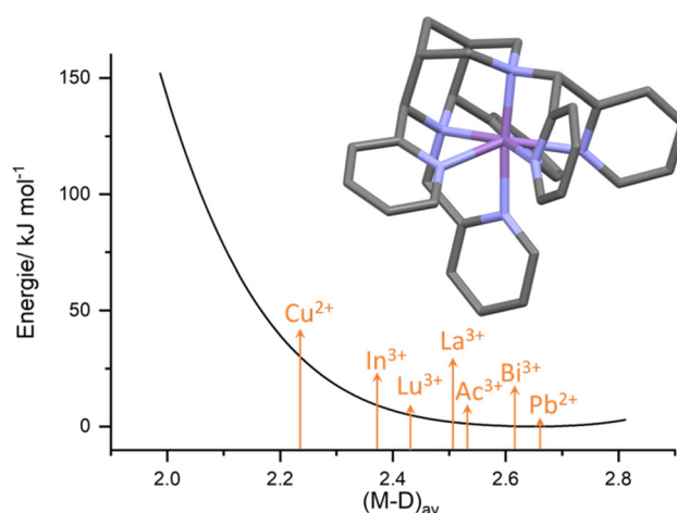
Fig. 3 Exemplary hole-size curve calculated for the heptadentate ligand L 6 (see Scheme 3 below). Arrows depict the approx. metal ion size ( i.e. , the average metal–donor distance for the appropriate metal ion – ligand combination) for a range of metal ions relevant for radiopharmaceutical applications. 16,22,42,55
