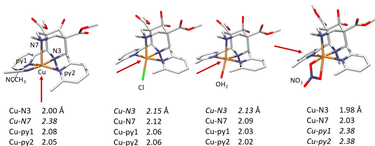
Fig. 2 Cu II complexes of the tetradentate 2,4-bis- \alpha -methylpyridyl substituted tetradentate bispidine L 2 , showing how the ligand-enforced tetragonal distortion may be varied by ligand substitution and choice of co-ligands (elongated bonds in italics ). 50
