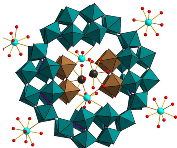
Fig. 18 Combined polyhedral/ball-and-stick representation of [K_{4.5}C(ClSn)_8P_8W_{48}O_{184}]^{17.5-} . Color code: WO_6 octahedra (green), PO_4 tetrahedra (pink), O (red), Sn (brown), K (grey), Cl (green). 129
