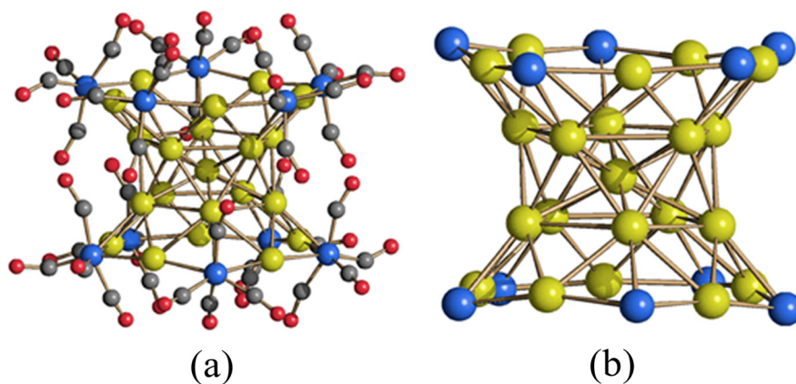
Fig. 28 Molecular structure (a) and metal core (b) of [Au 21 Fe 10 (CO) 40 ] 5- (yellow, Au; blue, Fe; grey, C; red, O). The central [Au 11 ] 5+ unit is bonded to two [Au 5 {μ-Fe(CO) 4 } 5 ] 5- rings containing linear Fe–Au–Fe motives.
