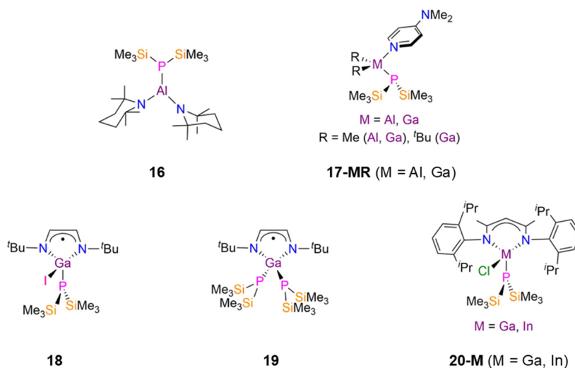
Fig. 5 Monomeric group 13 P'' complexes [Al(P'')(tmp) 2 ] (tmp = 2,2,6,6-tetramethyl-piperidino) ( 16 ), [M(R) 2 (P'')(dmap)] ( 17-MR . 17-AlMe : M = Al, R = Me; 17-GaMe : M = Ga, R = Me; 17-Ga t Bu : M = Ga, R = t Bu; dmap = 4-(dimethylamino)pyridine), [Ga(P'')(t) t Bu-DAB)] ( 18 , t Bu-DAB = {N( t Bu)C(H)} 2 ), [Ga(P'') 2 ( t Bu-DAB)] ( 19 ), [M(Diipp)(P'')(Cl)] (Diipp = {HC[C(Me)N(Dipp)] 2 , Dipp = C 6 H 5 Pr-2,6) ( 20-M ; M = Ga, In).
