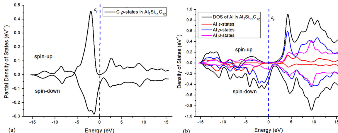
Fig. 3 The calculated PDOS from C (a), and Al (b) atoms for \text{Al}_x\text{Si}_{1-x}\text{C} NTs. Positive and negative DOS values represent majority and minority spin states, respectively.
