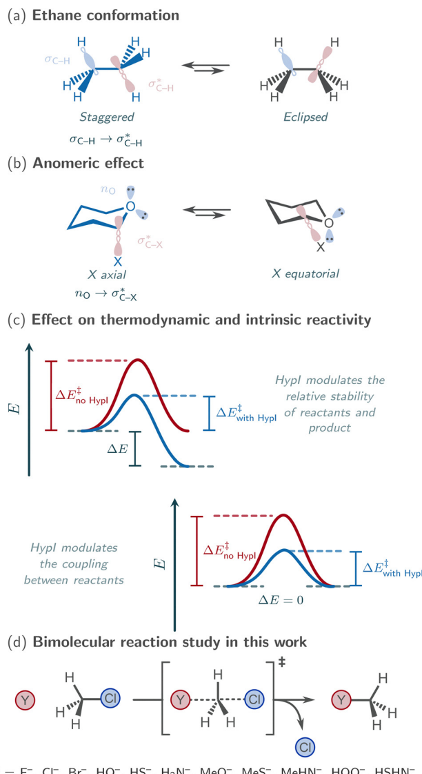
Fig. 1 (a) and (b) Representative configurational processes stabilized by hyperconjugative interactions (Hypl); the most stable conformers are highlighted in blue. (c) Conceptual illustration of how hyperconjugation can modulate both thermodynamic parameters (e.g., reaction energies) and intrinsic barriers. (d) Schematic representation of the S N 2 reaction under investigation, including the series of nucleophiles considered in this study.
