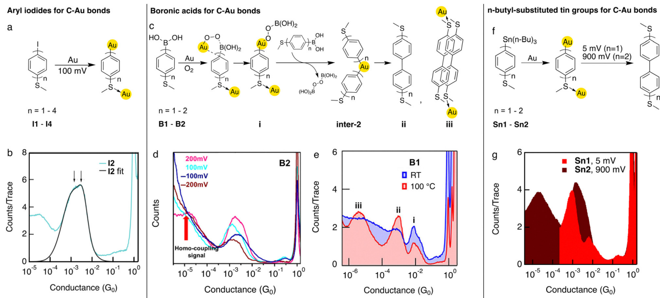
Fig. 3 (a) Schematic illustration of in situ cleavage of aryl iodides in forming junctions with C–Au covalent linkage on one side and a S \rightarrow Au dative bond on the other. (b) 1D histogram of I2 measured under 100 mV in TCB. The black line represents a double Gaussian fit to the data. (c) Proposed mechanism of in situ cleavage of the organoboron group, homocoupling reaction, and proposed molecular junction for the ultra-low conductance peak labeled as iii . (d) 1D conductance histograms of B2 measured under bias voltages of 200 mV, 100 mV, –100 mV, and –200 mV. (e) 1D conductance histograms of B1 measured in bis(2-ethylhexyl) adipate solvent under room temperature and 100 °C. (f) Schematic illustration of in situ cleavage of the organotin group and homocoupling reaction. (g) 1D conductance histograms of Sn1 and Sn2 measured in TCB under 5 mV and 900 mV bias voltages. (b) is adapted with permission from ref. 52, copyright (2020) American Chemical Society. (d) is adapted with permission from ref. 53, copyright (2022) Chinese Chemical Society. (e) is adapted with permission from ref. 54, copyright (2024) American Chemical Society. (g) is adapted with permission from ref. 57, copyright (2024) American Chemical Society.
