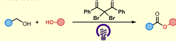
Scheme 1 Examples of photochemical cross-esterification reactions of alcohols.
