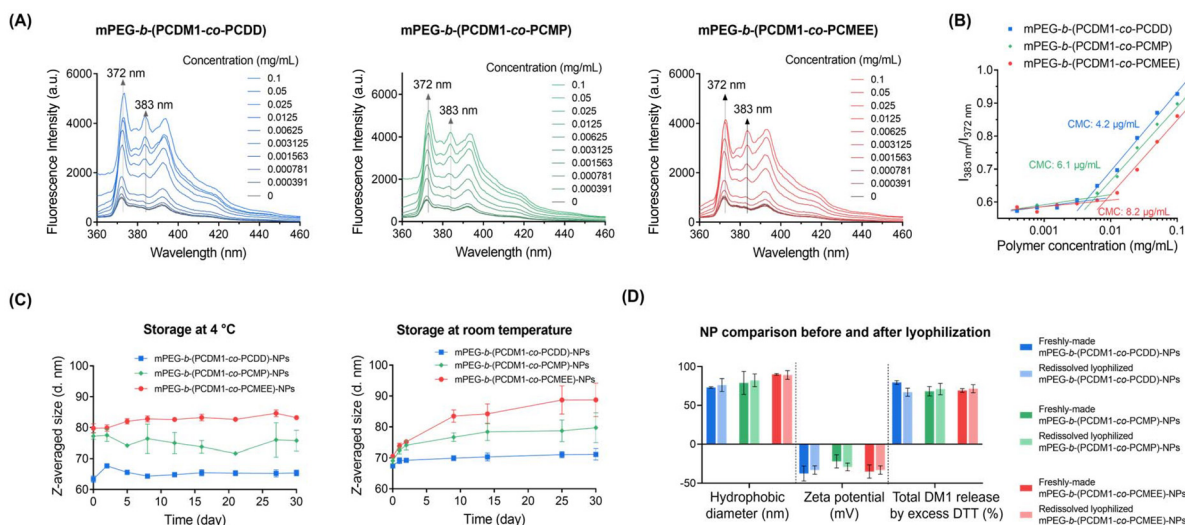
Fig. 4 (A) Fluorescence spectra of pyrene ( 0.12 \mu\text{g mL}^{-1} ) in the aqueous solutions of different concentrations of polycarbonate-DM1 conjugates ( 0\text{--}0.1 \text{ mg mL}^{-1} ): mPEG-b-(PCDM1-co-PCDD) (blue); mPEG-b-(PCDM1-co-PCMP) (green); and mPEG-b-(PCDM1-co-PCMEE) (red). (B) Fluorescence intensity ratio ( I_{383 \text{ nm}}/I_{372 \text{ nm}} ) of pyrene versus the logarithm concentration of polymers, with CMC determined by fitting the intensity ratio to identify the abrupt change point. (C) Long-term stability of self-assembled NPs at room temperature and under refrigerated conditions, evaluated by their Z-averaged size changes in DLS. (D) Comparison of sizes, zeta potentials, and DM1 release capabilities between the freshly made nanoparticles and reconstituted nanoparticles from lyophilized powders.
