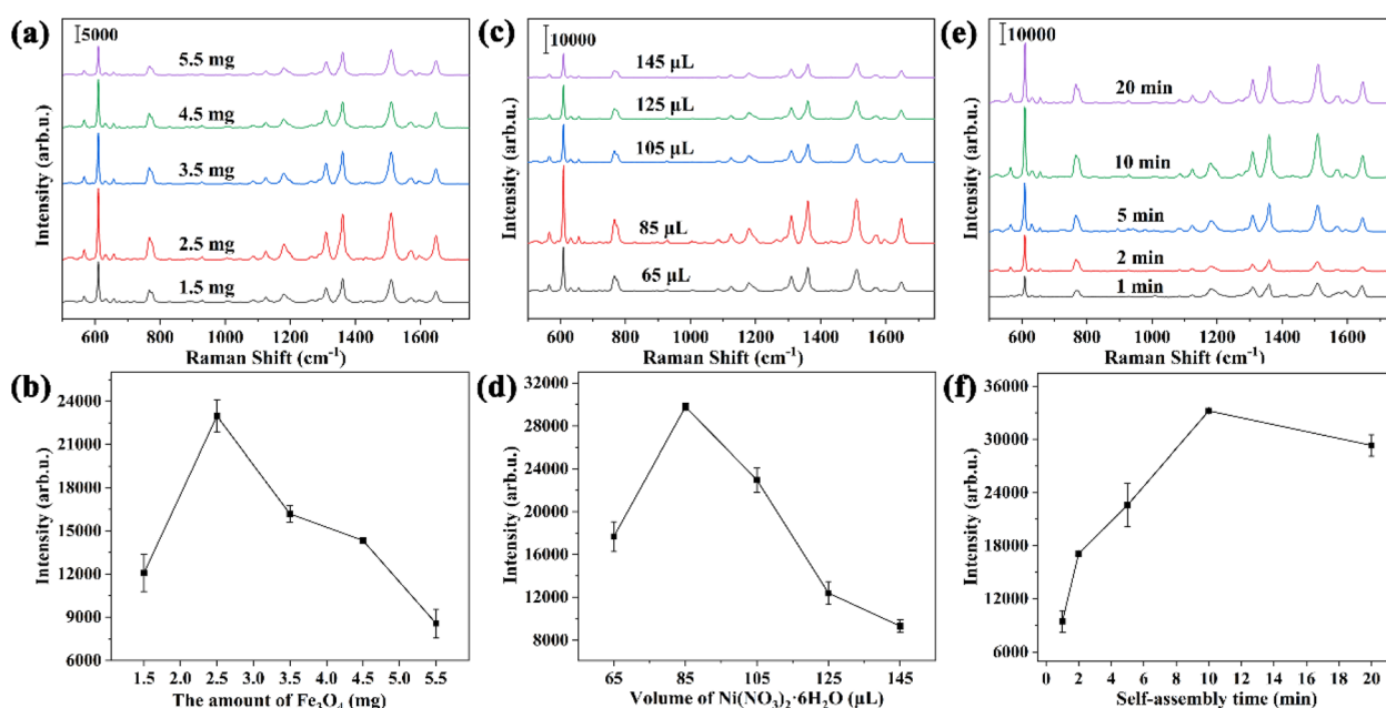
Fig. 3 (a) SERS spectra and (b) SERS intensity line chart at 612 \text{ cm}^{-1} of R6G ( 1 \times 10^{-6} \text{ mol L}^{-1} ) on the \text{Fe}_3\text{O}_4@\text{CoNi LDH}@\text{Ag} NP substrate with different amounts of \text{Fe}_3\text{O}_4 ; (c) SERS spectra and (d) SERS intensity line chart at 612 \text{ cm}^{-1} of R6G ( 1 \times 10^{-6} \text{ mol L}^{-1} ) on the \text{Fe}_3\text{O}_4@\text{CoNi LDH}@\text{Ag} NP substrate with different volumes of \text{Ni}(\text{NO}_3)_2 \cdot 6\text{H}_2\text{O} ; and (e) SERS spectra and (f) SERS intensity line chart at 612 \text{ cm}^{-1} of R6G ( 1 \times 10^{-6} \text{ mol L}^{-1} ) on the \text{Fe}_3\text{O}_4@\text{CoNi LDH}@\text{Ag} NP substrate with different self-assembly times.
