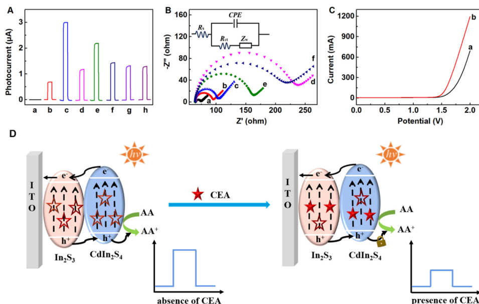
Fig. 4 (A) Photocurrent responses of the various modified electrodes: ITO (a), \text{In}_2\text{S}_3/\text{ITO} (b), \text{CdIn}_2\text{S}_4@/\text{ITO} (c), MIP/ \text{CdIn}_2\text{S}_4@/\text{ITO} (d), rMIP/ \text{CdIn}_2\text{S}_4@/\text{ITO} (e), IMIP/ \text{CdIn}_2\text{S}_4@/\text{ITO} (f), NIP/ \text{CdIn}_2\text{S}_4@/\text{ITO} (g), after the incubation of 100\text{ ng mL}^{-1} CEA (h). (B) EIS of the different electrodes: ITO (a), \text{In}_2\text{S}_3/\text{ITO} (b), \text{CdIn}_2\text{S}_4@/\text{ITO} (c), MIP/ \text{CdIn}_2\text{S}_4@/\text{ITO} (d), rMIP/ \text{CdIn}_2\text{S}_4@/\text{ITO} (e), and IMIP/ \text{CdIn}_2\text{S}_4@/\text{ITO} (f). Target concentration was 100\text{ ng mL}^{-1} . Inset: the electrical equivalent circuit applied to the fit the impedance data; R_s , Z_w , R_{ct} , and CPE represent the Ohmic resistance of the electrolyte, Warburg impedance, charge-transfer resistance, and constant phase angle element, respectively. (C) Current–voltage tests of \text{In}_2\text{S}_3/\text{ITO} (a) and \text{CdIn}_2\text{S}_4@/\text{ITO} (b). Electrolyte: 0.1\text{ M PBS} at \text{pH } 7.4 , scanning rate: 100\text{ mV s}^{-1} . (D) Photocurrent generation and regulation mechanisms of the designed MIP-PEC sensor.
