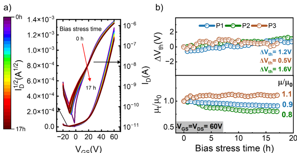
Fig. 4 (a) Transfer curves measured on OFETs of P1 films annealed at low temperatures (LTA) during 17 h of continuous bias stress at V_{\text{GS}} = V_{\text{DS}} = 60 \text{ V} . (b) Evolution of threshold voltage and mobility normalised to its value at t = 0 with time for n-type OFETs upon continuous bias stress at V_{\text{GS}} = V_{\text{DS}} = 60 \text{ V} .
