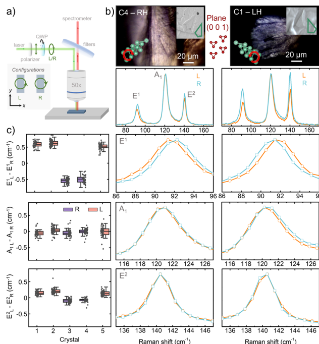
Fig. 3 Circularly polarized Raman characterization of representative right- and left-handed bulk Te crystals carried out falling upon the (0 0 1) crystallographic plane: (a) sketch of the circularly polarized Raman measurements showing the optical elements for this configuration using incident circularly polarized light and collecting unpolarized signal. (b) Optical images taken with the micro-Raman instrument of the crystal faces under study accompanied by representative Raman spectra showing the characteristic Raman modes ( E^1 , A_1 and E^2 ) obtained using right- (R, blue) and left- (L, orange) handed light excitation (below). The insets show images of the corresponding etch pit indicating that the Te crystals handedness: right (C4) and left (C1). The panels below present zoomed ranges of the normalized Raman spectra making more visible the E phonon doublet shift while A_1 phonon does not change. (c) Box and scatter plots (dots display the data collected) for the phonons shift under right- and left-handed light excitation for the five crystals under study: left-handed (C1, C2, C5) (pink) and right-handed (C3, C4) (purple).
