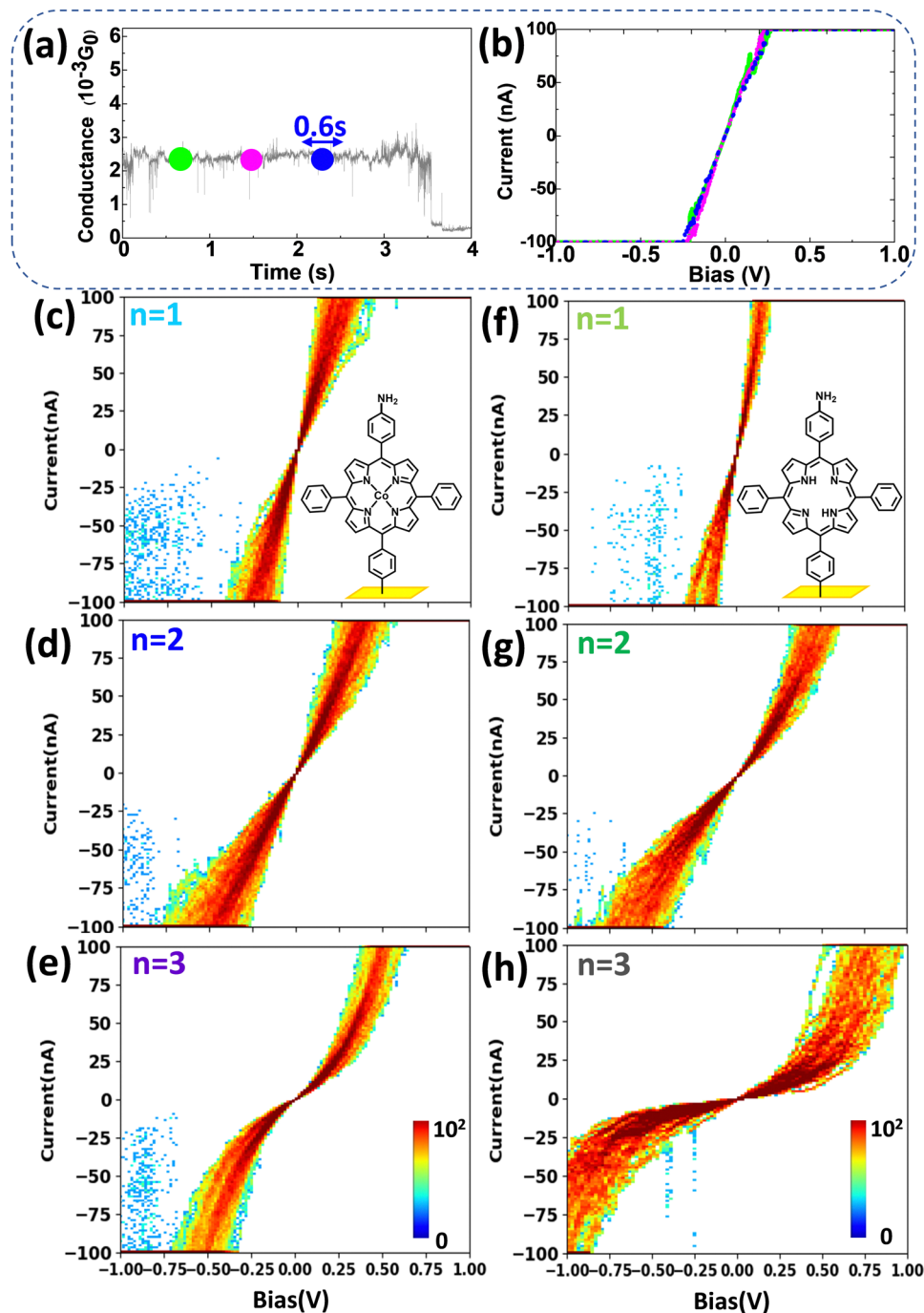
Fig. 4 In-depth I/V characteristics of SMJs: (a) typical \text{Au}-[\text{CoTPP}]_1-\text{Au} G(t) trace; the colored dots indicate the 0.6 s time for an I/V measurement. (b) Three different I/V traces from junctions of (a). 2D I/V heat maps for (c)–(e) \text{Au}-[\text{CoTPP}]_n-\text{Au} and (f)–(h) \text{Au}-[\text{TPP}]_n-\text{Au} junctions of different lengths, n = 1, 2, 3 , respectively.
