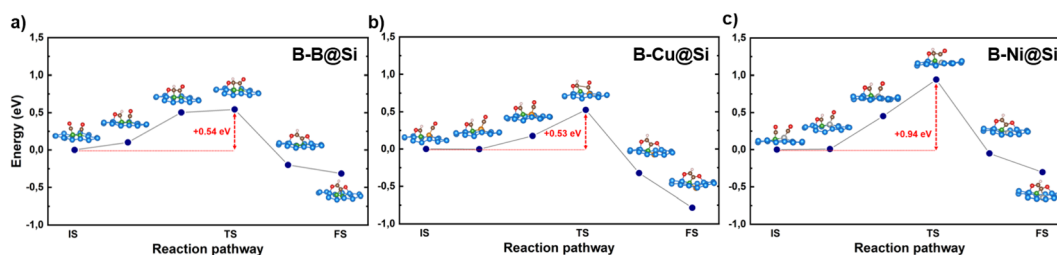
Fig. 4 The reaction path energy diagrams for the coupling step \text{CHO}-\text{CO}^* \rightarrow \text{OCHCO}^* on (a) B–B@Si, (b) B–Cu@Si and (c) B–Ni@Si. The insets show the atomic structures of initial state (IS), transition state (TS) and final state (FS). Red numbers indicate the activation energy barriers. Color code: B – green, Cu – orange, Ni – silver, Si – light blue, C – brown, O – red and H – light pink.
