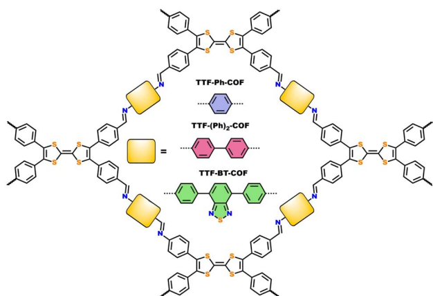
Scheme 1 Schematic representation of the three 2D TTF-COFs.
