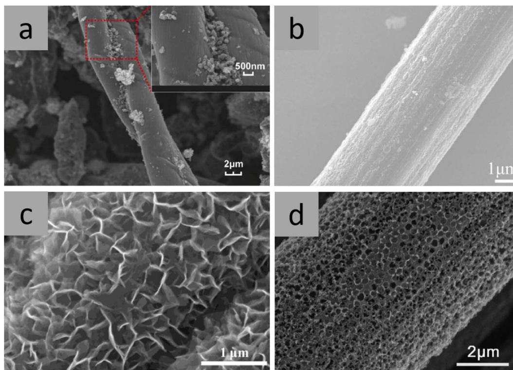
Fig. 6 Scanning electron microscopy (SEM) images of CFBA with different coating morphologies, including (a) inhomogeneous MnO, 45 (b) homogeneous Co 3 O 4 , 21 (c) V 2 O 5 nanosheets, 53 and (d) macroporous MoS 2 . 54 The void spaces in the MoS 2 coating were created by including polystyrene spheres in the coating that thermally decompose during annealing, demonstrating a creative use of the annealing process during the coating step. (a) Reproduced from ref. 45 with permission from Elsevier, copyright 2024. (b) Reproduced from ref. 21 with permission from Springer Nature, copyright 2024. (c) Reproduced from ref. 53 with permission from Elsevier, copyright 2024. (d) Reproduced from ref. 54 with permission from Wiley, copyright 2024.
