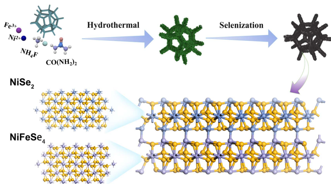
Fig. 1 Synthesis process of \text{NiFeSe}_4/\text{NiSe}_2 .
