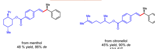
Scheme 16 Dual Ir/nickel-catalyzed synthesis for stereo- and enantio-selective benzylic \text{C(sp}^3\text{)} –H alkenylation.
