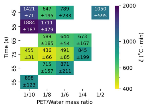
Fig. 6 Effect of batch holding time and m_{\text{PET}}/m_{\text{w}} on the environmental energy impact metric from fast hydrolysis of post-consumer PET at T_{\text{SP}} = 510^\circ\text{C} .
