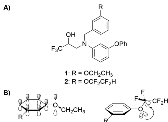
Fig. 1 (A) The structures of CETP inhibitors reported by Durley and co-workers. 19 The non-fluorinated analogue 1 has a IC 50 of 1.6 \mu M while the fluorinated analogue 2 has an IC 50 of 0.2 \mu M. The values were determined in a buffer transfer assay. (B) Hyperconjugative \pi - \sigma^* C-F interaction rationale for the reduced in-plane conformational preference of a fluoroalkoxyaryl group. 19
