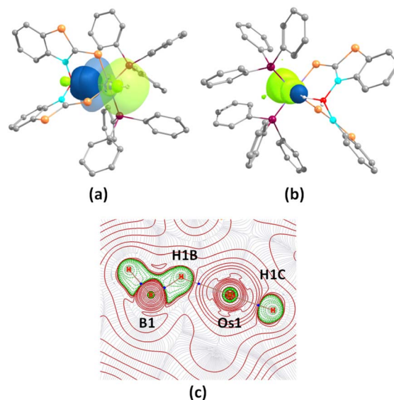
Fig. 6 (a) Donor–acceptor interaction between \sigma(\text{B–H}) and the Os center in 4a ; (b) Os–H bonding interaction in 4a (isovalue 0.004 [ e bohr ^{-3} ] ^{1/2} ); (c) contour-line diagram of the Laplacian of the electron density along Os–H–B planes in 4a .
