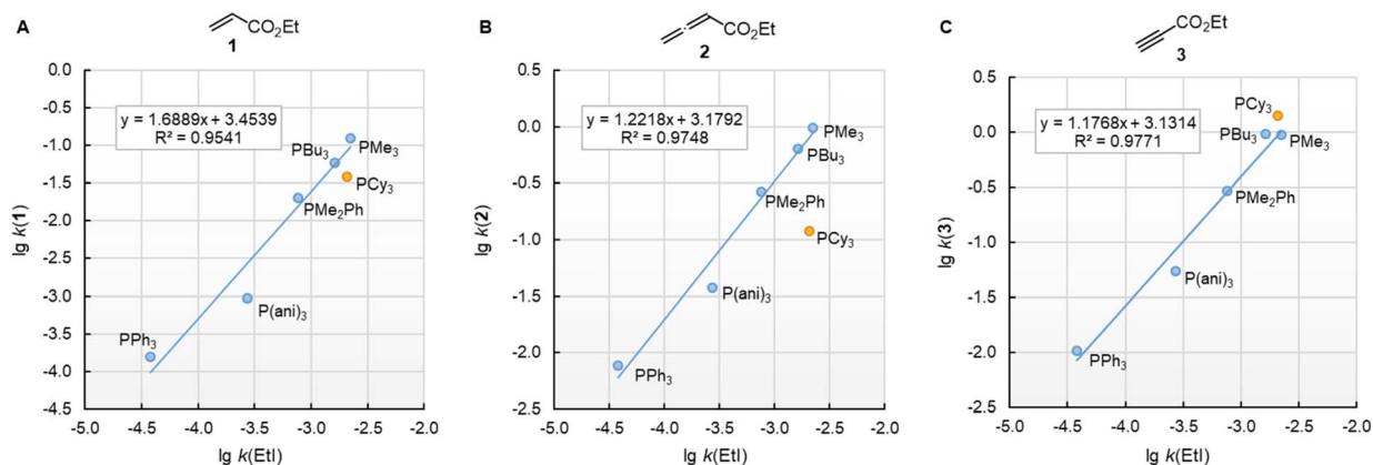
Fig. 7 Reactivities ( \lg k_2 ) of \text{PR}_3 towards (A) ethyl acrylate (1), (B) ethyl allenolate (2), and (C) ethyl propiolate (3) correlate linearly with the S_N2 reactivity of \text{PR}_3 towards ethyl iodide (in acetone at 35 °C, ref. 29b). With rate constants k_2 from Table 3, data for the sterically encumbered \text{PCy}_3 excluded when constructing the correlation lines.
