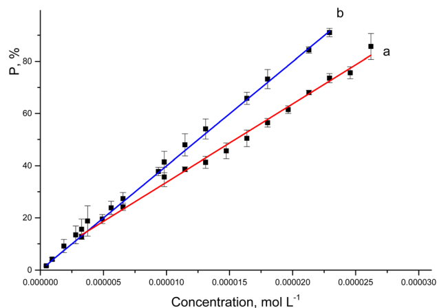
Fig. 8 The correlation equations between the percentage of DPPH radical scavenging activity of rutin (a) or [Rut\subset\beta\text{-}CD] (b) and their concentrations.
