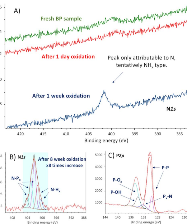
Fig. 2 (A) N1s X-ray photoelectron spectra (XPS) of fresh FL-BP (green line), and left under ambient conditions for 1 day (red line) and 1 week (blue line) respectively, managed and recorded at HIERN laboratory. (B) Deconvoluted high-resolution N1s XPS of FL-BP left under ambient conditions for 8 weeks, managed and recorded at ITQ-UPV/CSIC laboratory. (C) Deconvoluted high-resolution P2p XPS of the previous sample (B).
