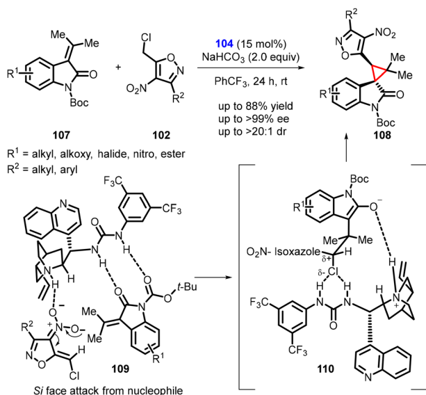
Scheme 21 Asymmetric cyclopropanation of N - boc -isopropylidene oxindole and 5-(chloromethyl)-3-methyl-4-nitroisoxazole.
