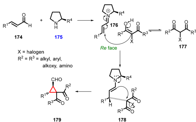
Scheme 36 Proposed mechanism for the cyclopropanation of enals with halocarbonyl compounds.
