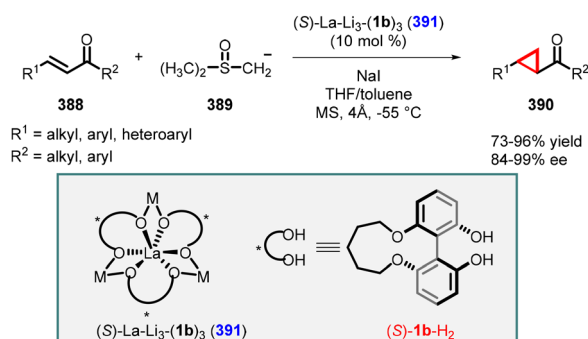
Scheme 86 \text{La-Li}_3 -(biphenyldiolate) _3/\text{NaI} complex catalyzed MIRC cyclopropanation of enones with dimethyl-oxosulfonium methylide.
