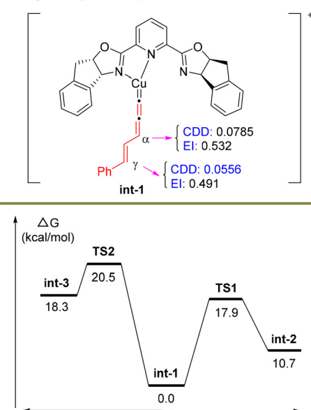
Scheme 4 Preliminary mechanistic studies. BP86/def2tzvp/SMD(methanol)//B3LYP-D3(BJ)/6-31g*/SDD was used for DFT calculations.
