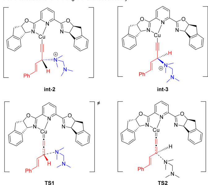
Scheme 4 Preliminary mechanistic studies. BP86/def2tzvp/SMD(methanol)//B3LYP-D3(BJ)/6-31g*/SDD was used for DFT calculations.
