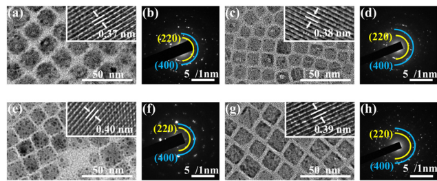
Fig. 2 TEM and HRTEM images (insets) of (a) \text{Cs}_2\text{AgInCl}_6 , (c) 2%Bi, (e) 20%Yb, 7%Er and (g) 2%Bi@20%Yb, 7%Er NCs, and their corresponding SAED patterns (b, d, f and h). Some 'dark dots' appearing in the TEM images over the surface of the NCs are attributable to the reduction of \text{Ag}^+ to \text{Ag}^0 by Olam. 21,34
