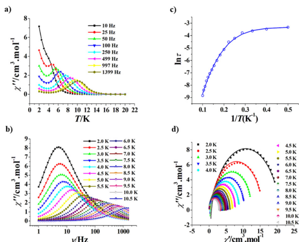
Fig. 7 Plots of \chi'' versus T for D-2 ( H_{\text{dc}} = 0 Oe) (a). Frequency dependence of \chi'' for D-2 at a zero dc field (b). Plot of \ln(\tau) versus 1/T for D-2 ( H_{\text{dc}} = 0 Oe); the solid line represents the best fitting with quantum tunnelling plus Orbach plus Raman (c). Cole–Cole plots measured from 2.0 to 10.5 K for D-2 ( H_{\text{dc}} = 0 Oe); the solid lines represent the best fitting with the generalized Debye model (d).
