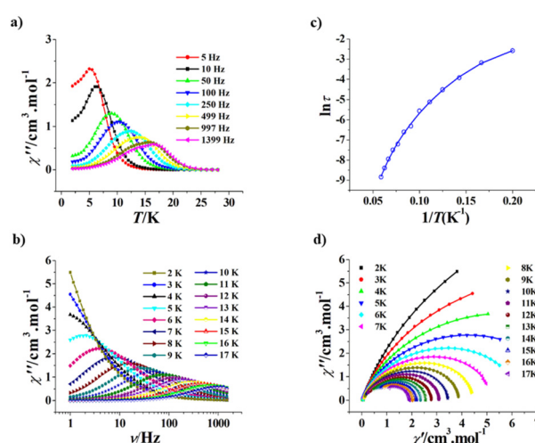
Fig. 8 Plots of \chi'' versus T for D-3 ( H_{\text{dc}} = 0 Oe) (a). Frequency dependence of \chi'' for D-3 at a zero dc field (b). Plot of \ln(\tau) versus 1/T for D-3 ( H_{\text{dc}} = 0 Oe); the solid line represents the best fitting with quantum tunnelling plus Orbach plus Raman (c). Cole–Cole plots measured from 2.0 to 17 K for D-3 ( H_{\text{dc}} = 0 Oe); the solid lines represent the best fitting with the sum of two modified Debye functions (d).
